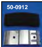
50-0912 Chrome Rear Fender Bracket fits 1954-78, reduces vibration between fender and frame, includes foam pad, replaces 59795-52A. VT No. Item 50-0912 Bracket with pad 28-2246 Foam pad only
