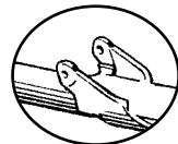
VT No. Item 31-4024 Complete Kit, All 13-1952 4 Springs, Set (A and B) 13-9173 Swivel Springs, Pin, (F) 37-9114 Tee Bolt, (C) 10-2564 Bushing, (D) 10-2563 Spacer, (E) 31-4083 Kit with Tee
