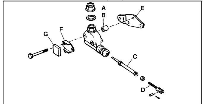
Rear Master Cylinder Hardware.
