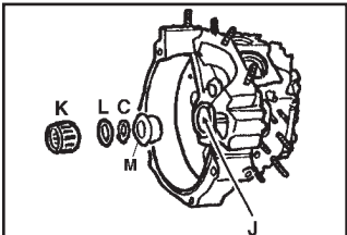
Right Crankcase Bearing and Spacers for 1958-99 Big Twin models.
